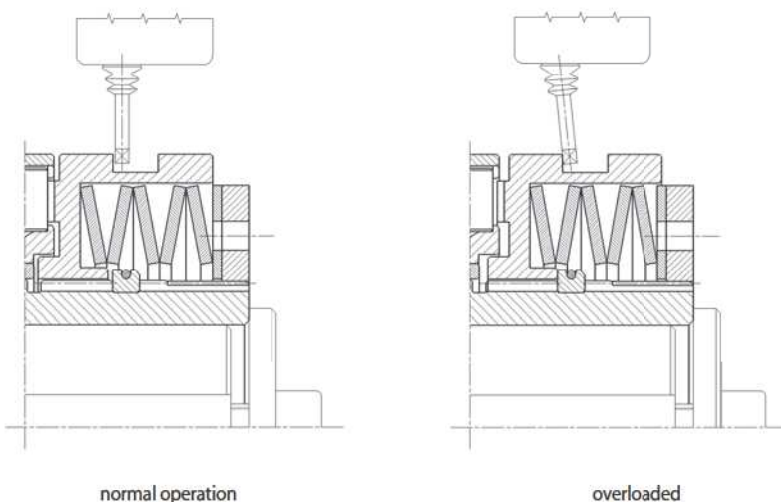
Overload signal
