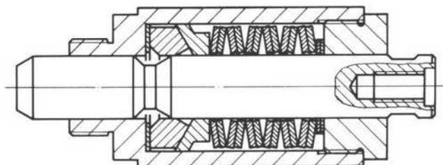
Series PA without proximity switch
